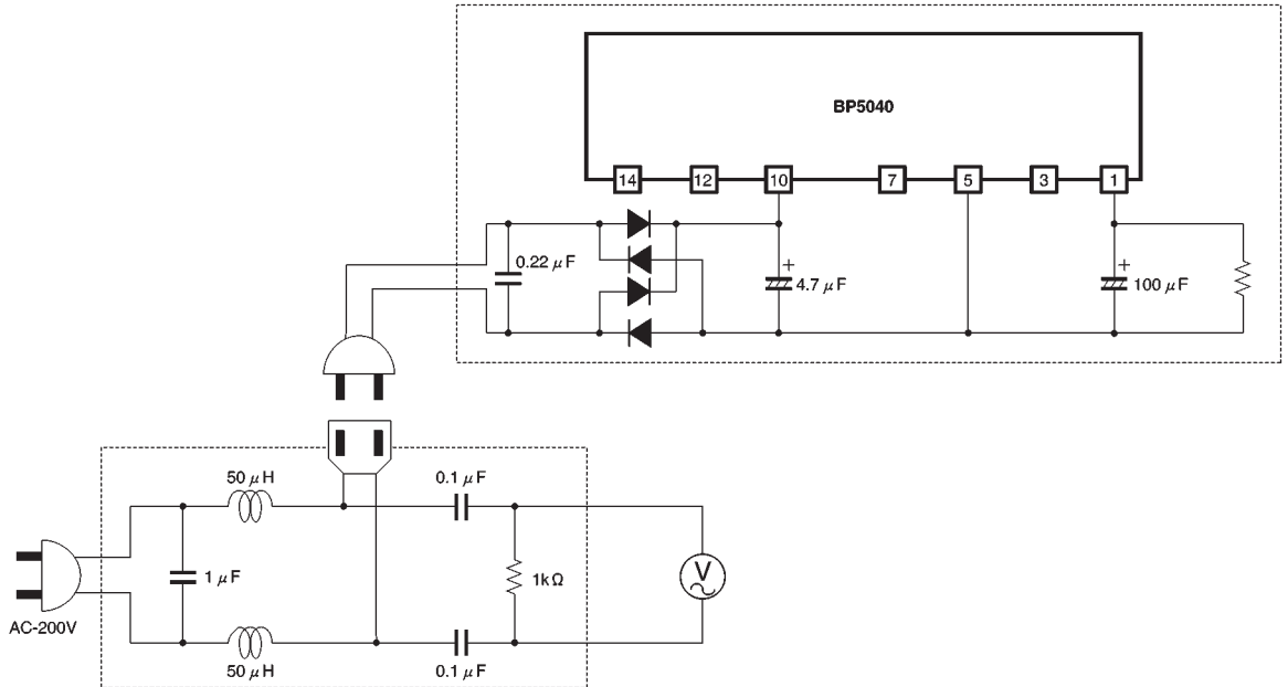
Fig.6 Test circuit
