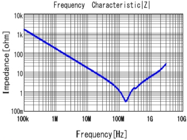
■ GA242QR7E2102MW01 |Z| DCOV, 25degC
