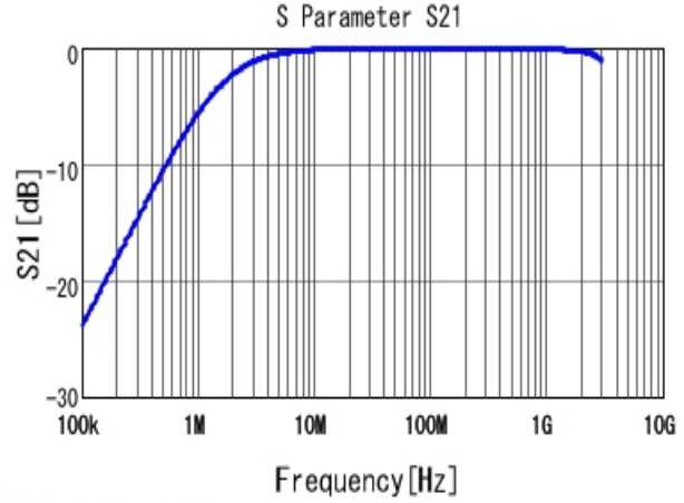
■ GA242QR7E2102MW01 S21 DCOV, 25degC
