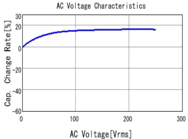
■ GA242QR7E2102MW01 C-AC Voltage capchange, DCOV, 25.0d
