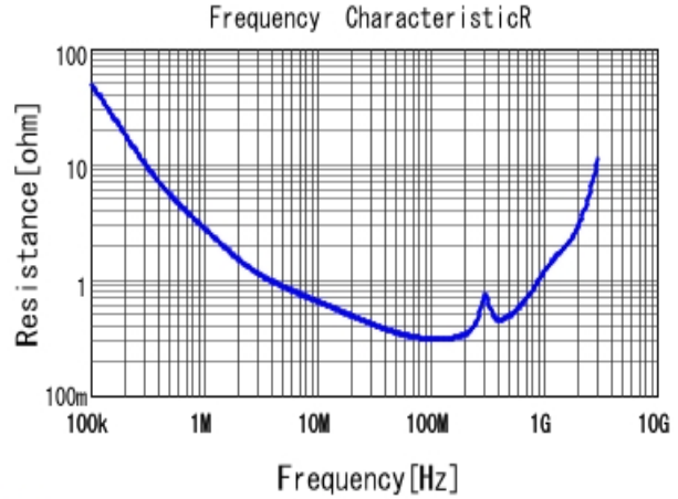
■ GA242QR7E2102MW01 R DCOV, 25degC
