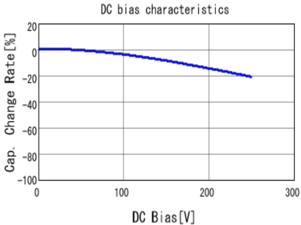
■ GA242QR7E2102MW01 C-DC bias capchange, 25.0degC, AC1V
