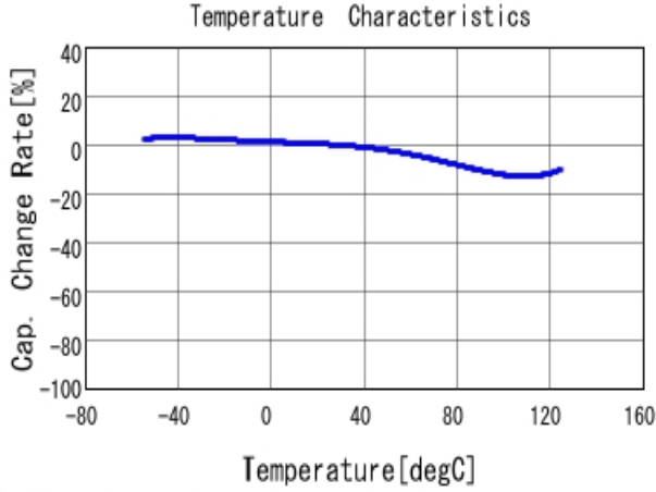
■ GA242QR7E2102MW01 C-Temp. capchange, DCOV, AC1Vrms
